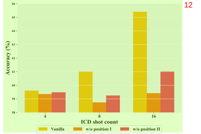
Figure 7: Average performance comparison of CAMA (Vanilla vs. w/o position-decay factors) under different shot counts.
